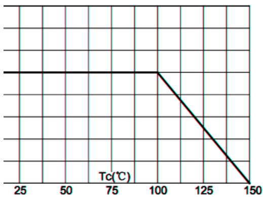
3: Forward current vs. case temperature
