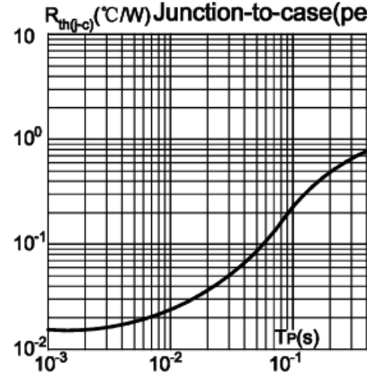
FIG.4: Maximum transient thermal
