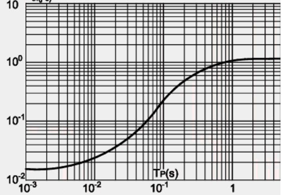
FIG.4: Maximum transient thermal impedance R_{th(j-c)} ( ^\circ\text{C/W} ) Junction-to-case(per diode)
