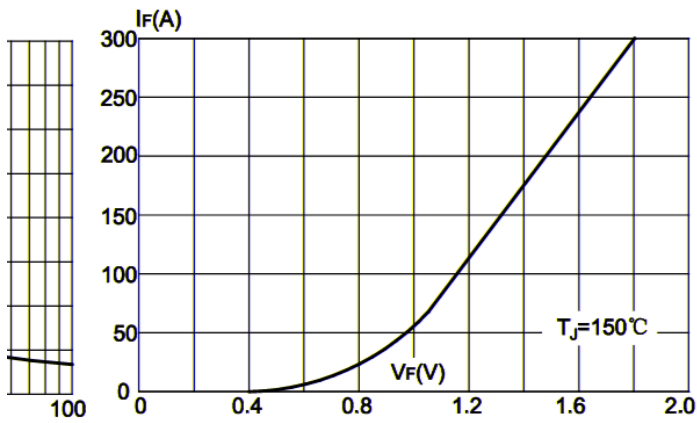
FIG.1: Forward characteristics(per diode)
