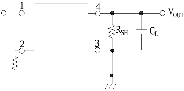
FIG.7: Response Time Test Circuit, Waveform
