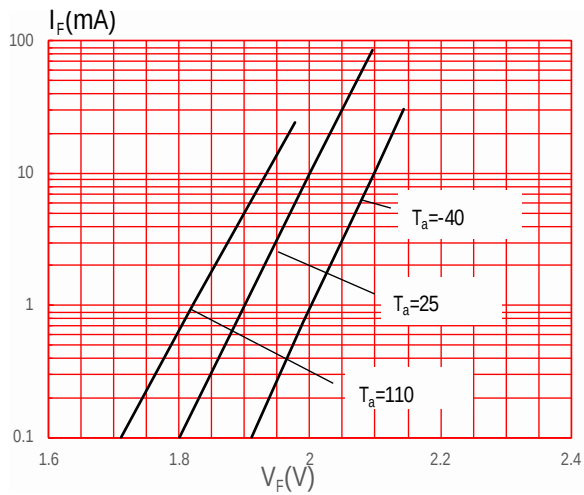
LED Forward Current vs. LED Dropout Voltage
