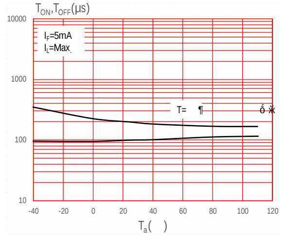
T_{ON}, T_{OFF} vs. Ambient Temperature
